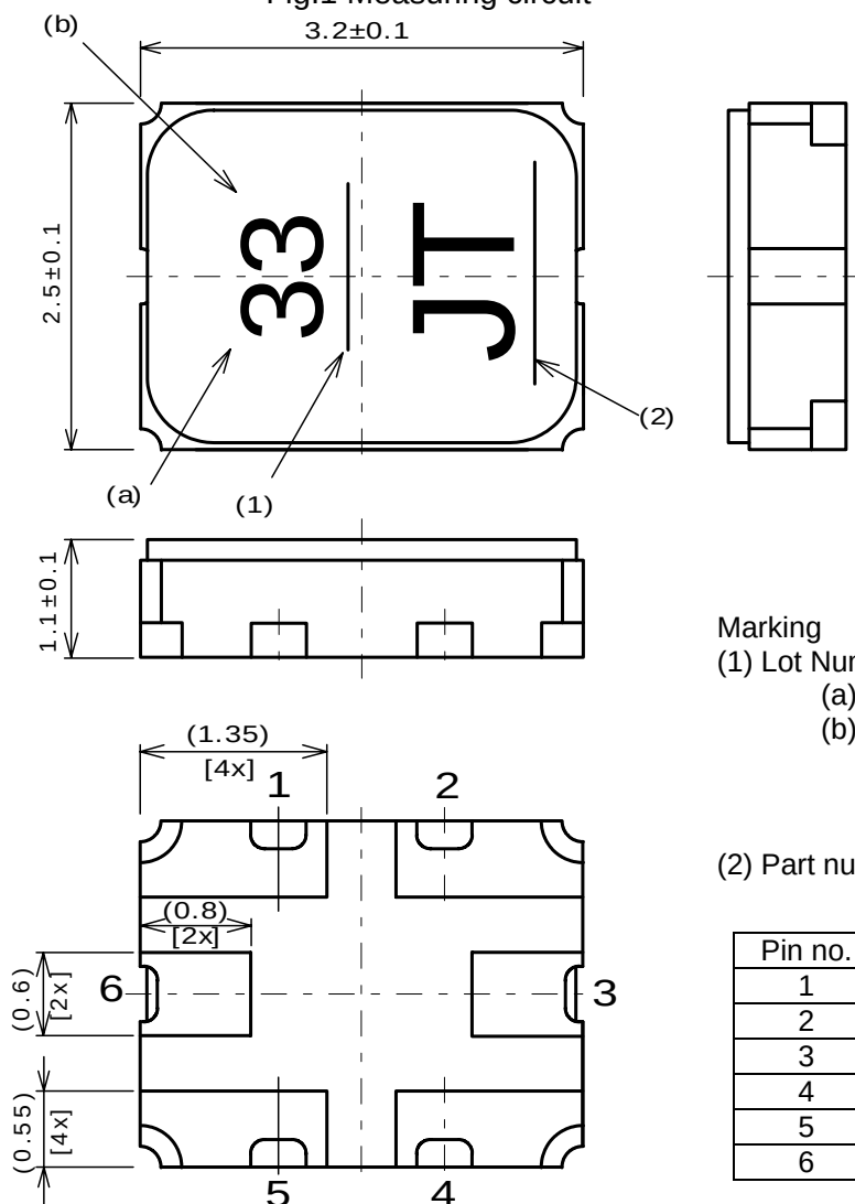
Fig.2 Package dimensions (in mm)
